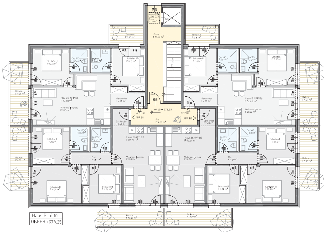
Building B - Top floor
