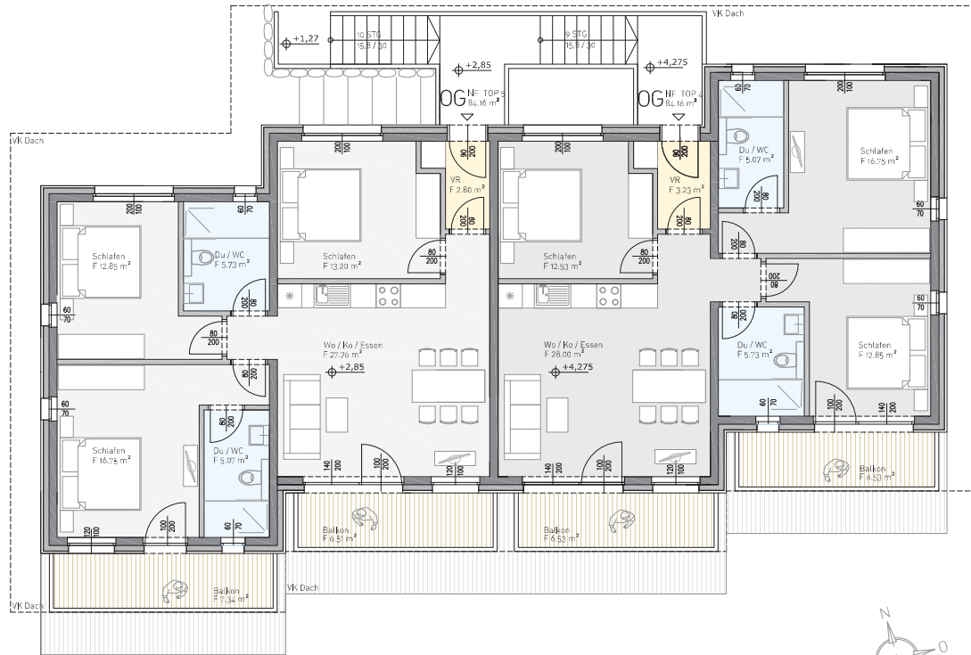
Top floor
