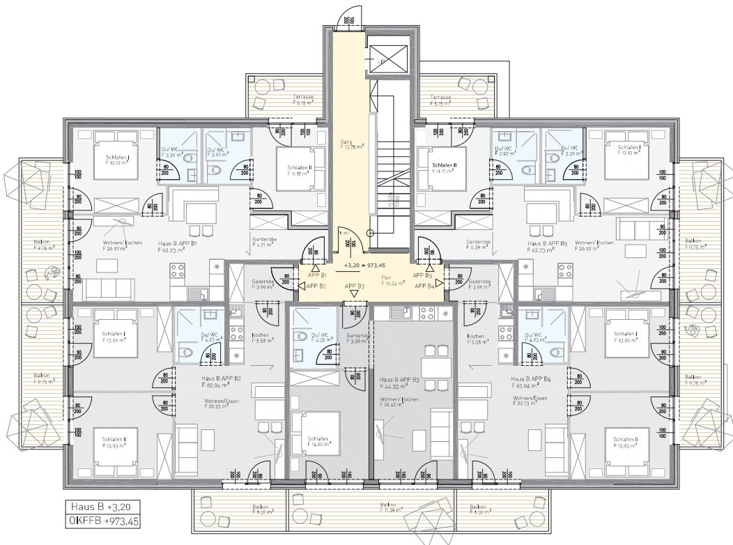
Building B - First floor
